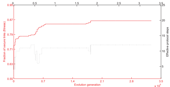
Figure 9: The typical progress of the fitness value and the number of effective instructions of the group-oriented protocol for one evolution run. Solid line shows fitness value (fraction of secure links) for the best candidate protocol in the particular generation and dotted line shows the number of effective protocol steps (after pruning) of the best candidate.
